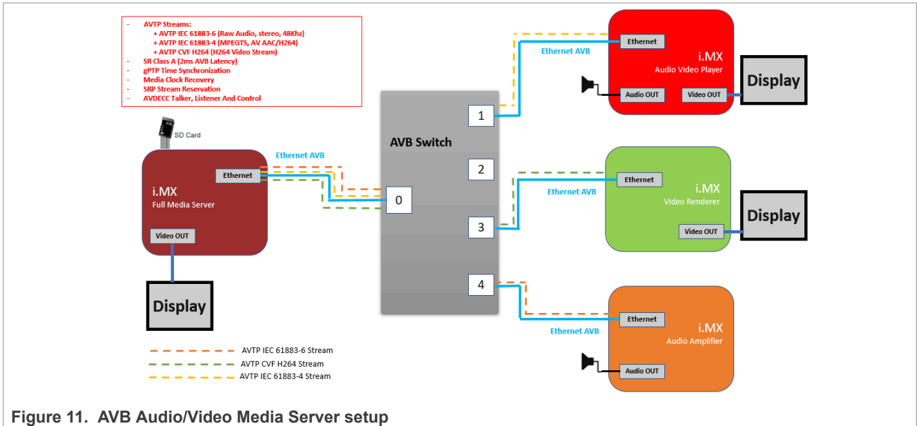
Figure 11. AVB Audio/Video Media Server setup
