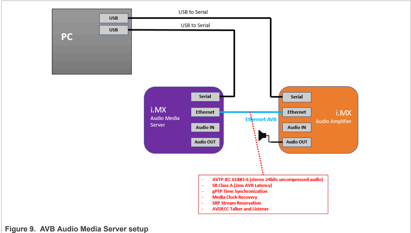
Figure 9. AVB Audio Media Server setup
