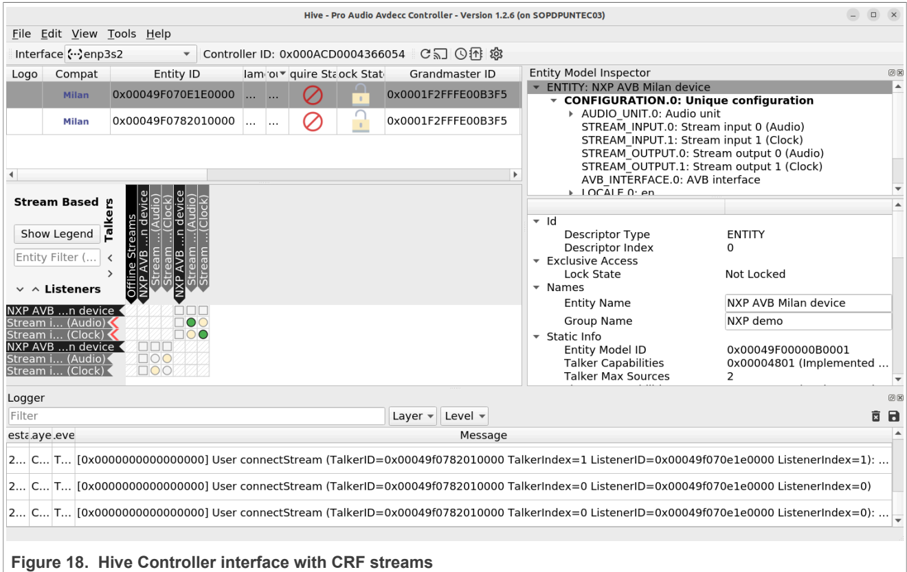
Figure 18. Hive Controller interface with CRF streams
