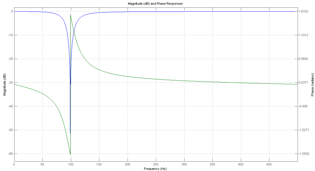
Figure 36. Filter response
