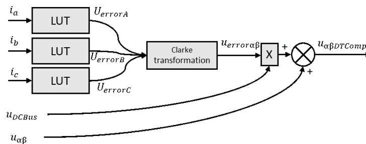
Figure 26. GMCLIB_DTCompLut1D function block scheme
