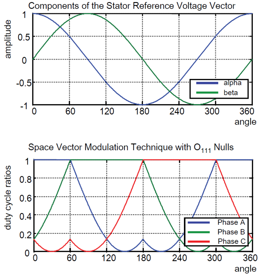
Figure 55. Space vector modulation technique with O_{111} nulls
