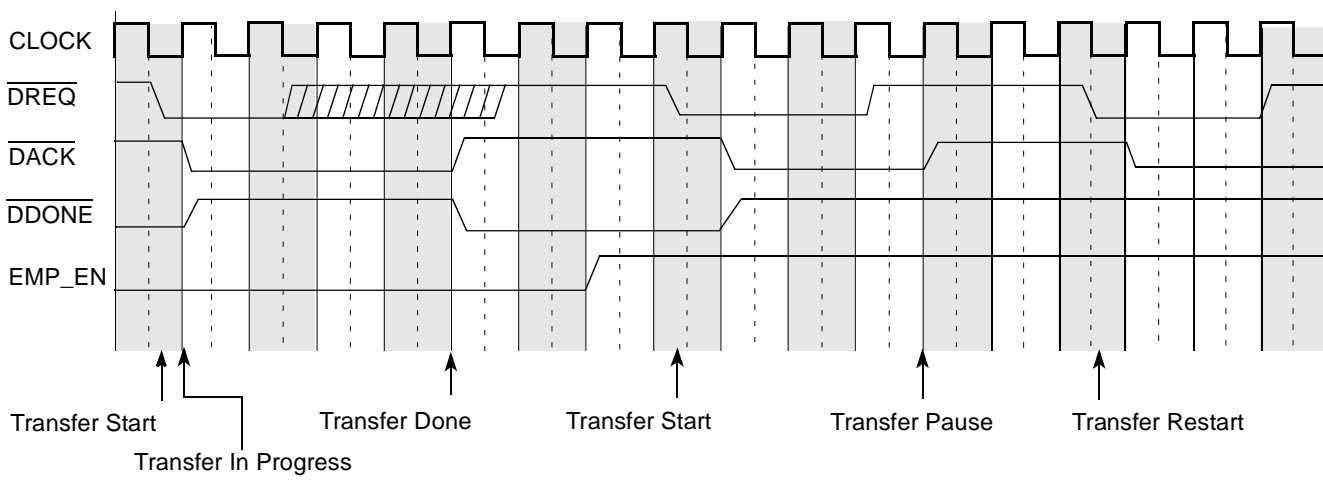
Figure 15-22. External Control Interface Timing
