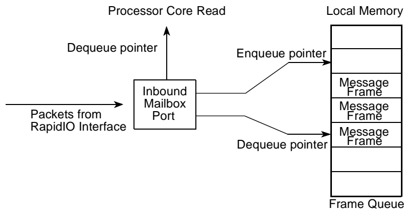
Figure 17-84. Inbound Mailbox Structure
