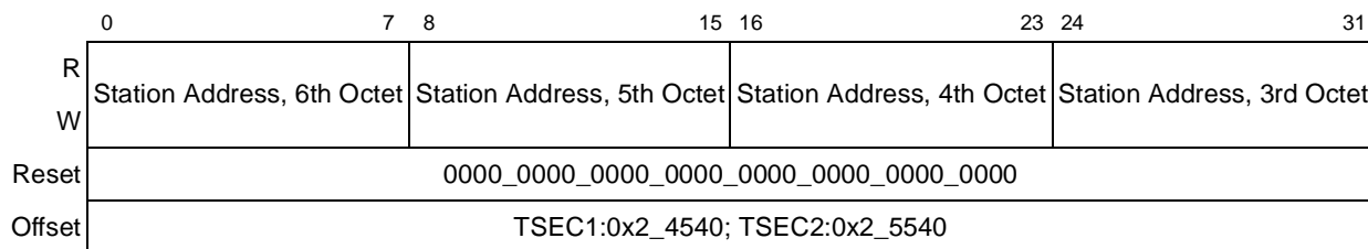
Figure 14-47. Station Address Part 1 Register Definition
