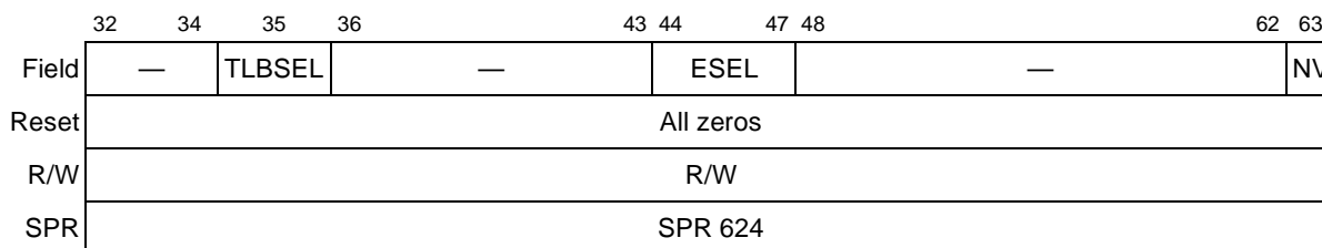
Figure 6-42. MAS Register 0 (MAS0)
