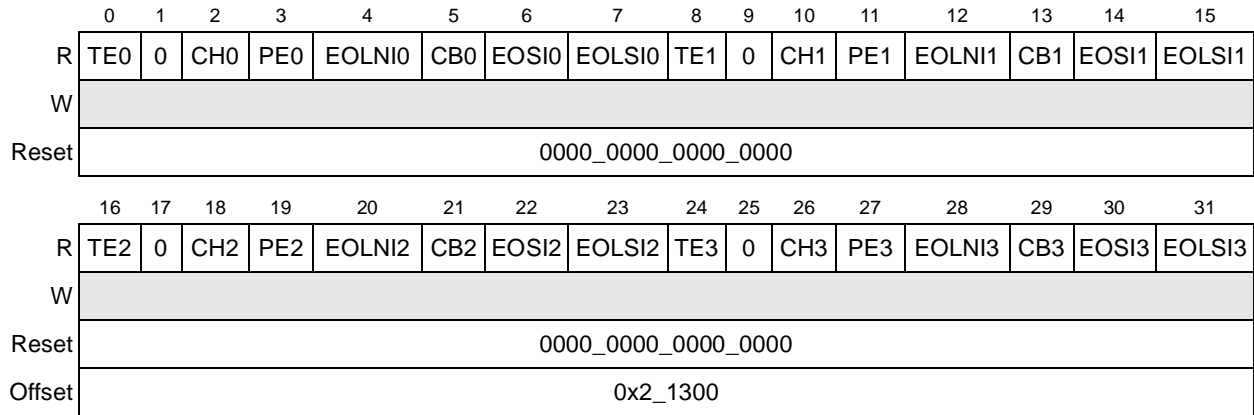
Figure 15-21. DMA General Status Register (DGSR)
