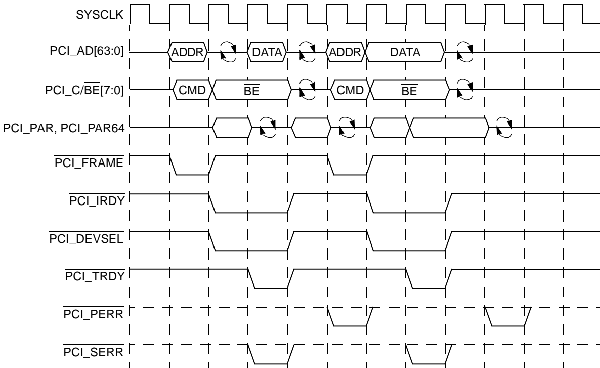
Figure 16-67. PCI Parity Operation
