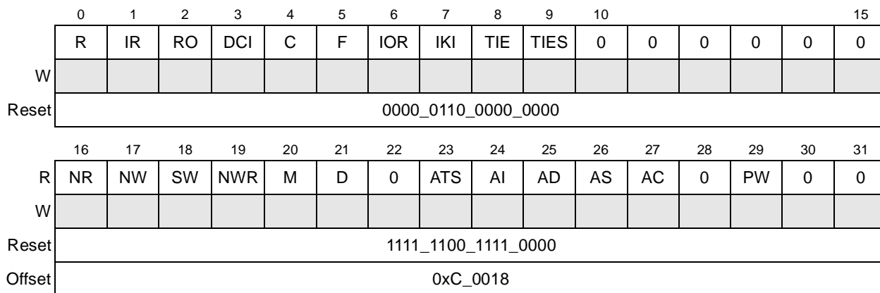
Figure 17-9. Source Operations Capability Register (SOCAR)
