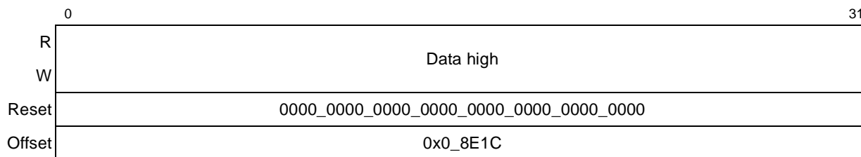
Figure 16-22. PCI/X Error Data High Capture Register (ERR_DH)
