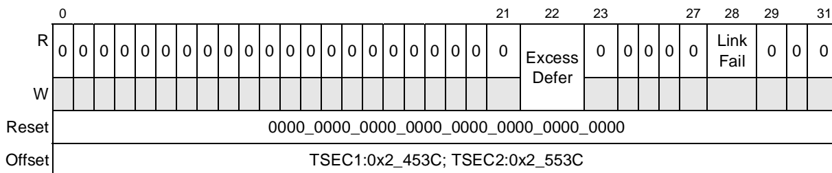
Figure 14-46. Interface Status Register Definition
