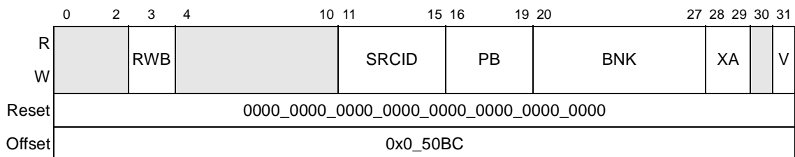
Figure 13-16. Transfer Error Attributes Register (LTEATR)
