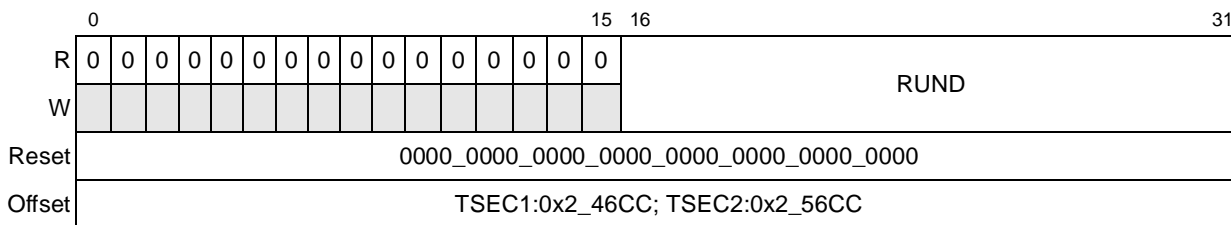
Figure 14-68. Receive Undersize Packet Counter Register Definition
