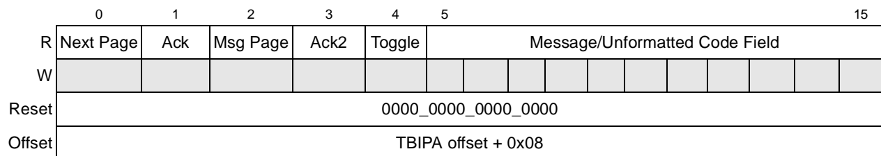
Figure 14-106. AN Link Partner Ability Next Page Register Definition
