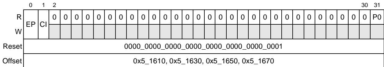
Figure 10-30. Messaging Interrupt Destination Registers (MIDR n )
