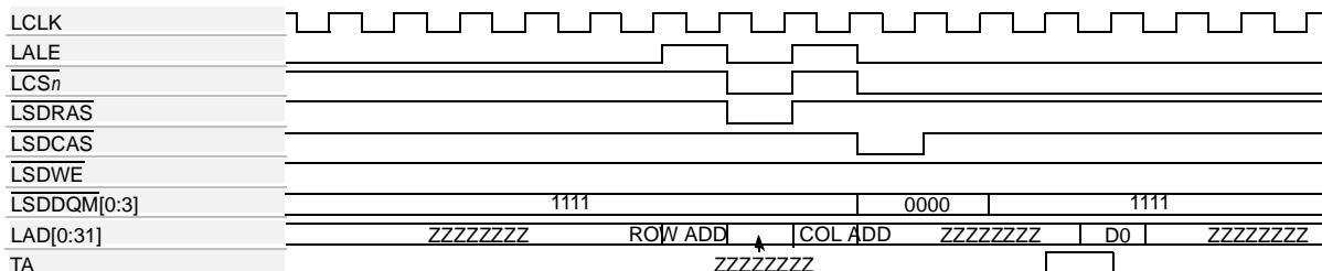
Figure 13-41. SDRAM Single-Beat Read, Page Closed, CL = 3
