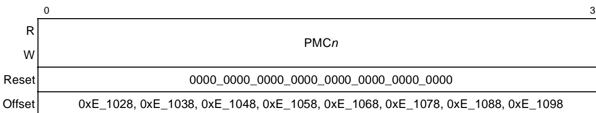
Figure 19-8. Performance Monitor Counter Registers 1–8 (PMC1–PMC8)
