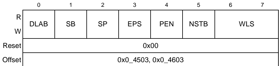
Figure 12-9. Line Control Register (ULCR)
