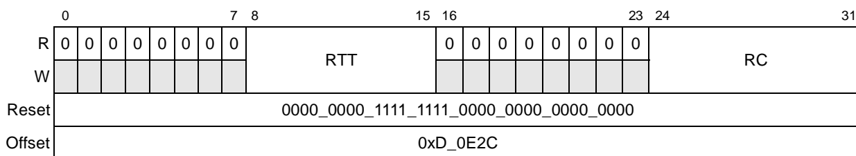
Figure 17-61. Port Retry Threshold Register (PRTR)
