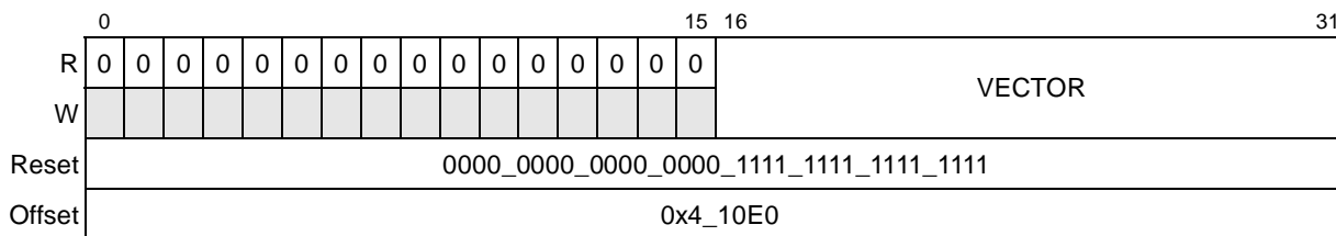
Figure 10-8. Spurious Vector Register (SVR)
