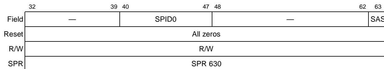
Figure 6-47. MAS Register 6 (MAS6)
