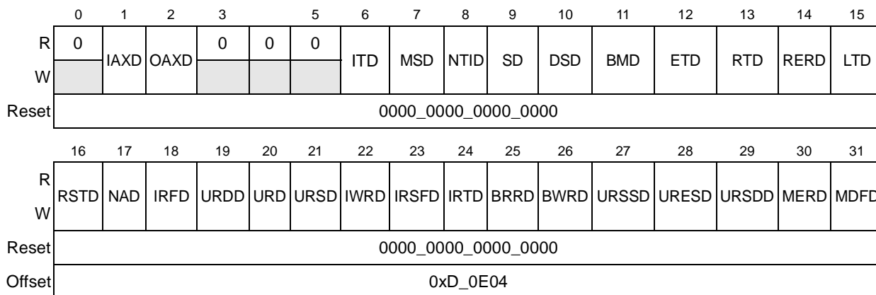
Figure 17-40. Port Notification/Fatal Error Detect Disable Register (PNFEDiR)
