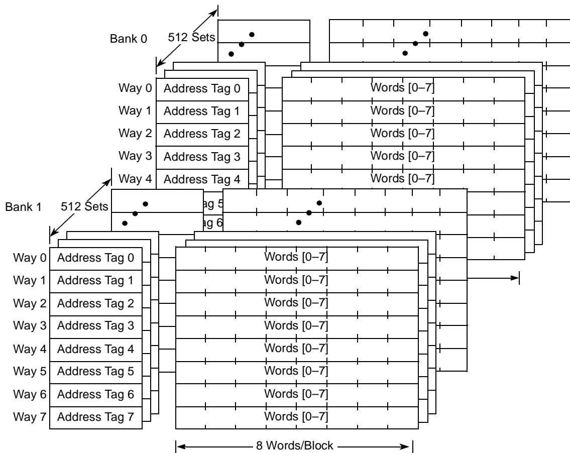
Figure 7-2. Cache Organization
