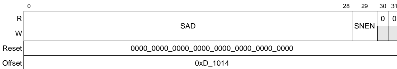
Figure 17-65. Outbound Unit Source Address Registers (OSAR)
