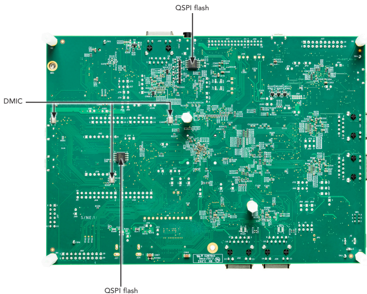
Figure 2: MIMXRT1180-EVK board back callouts
