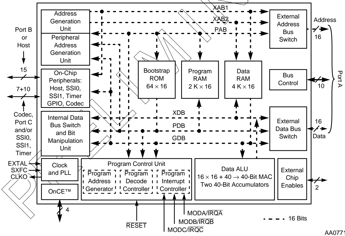
Figure 1 DSP56167 Block Diagram
