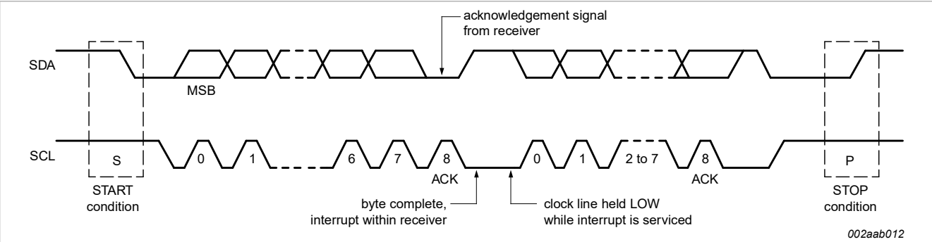
Figure 19. Data transfer on the I 2 C-bus
