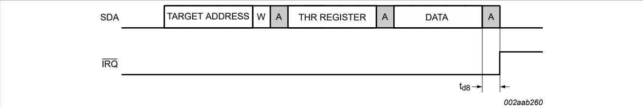
Figure 33. Transmit interrupt clear
