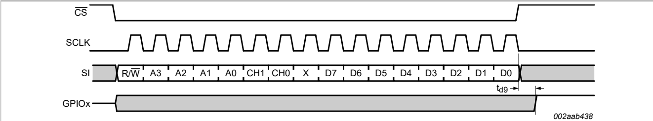
Figure 35. Detailed SPI-bus timing
