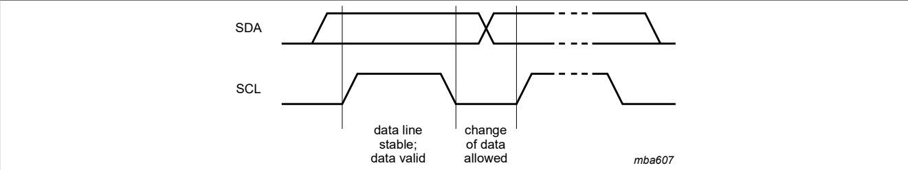
Figure 17. Bit transfer on the I 2 C-bus
