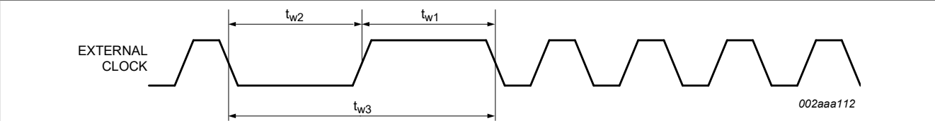
Figure 34. External clock timing
