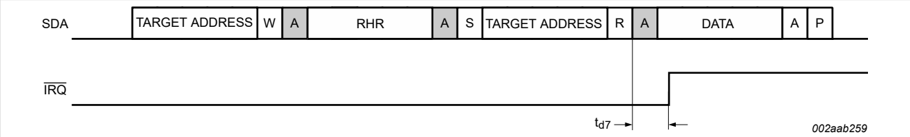
Figure 32. Receive interrupt clear
