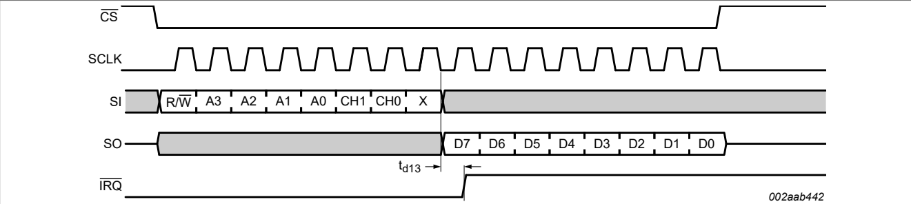
Figure 39. Read MSR to clear modem INT (SC16IS750 and SC16IS760 only)
