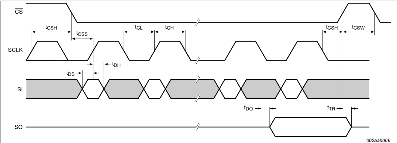
Figure 35. Detailed SPI-bus timing
