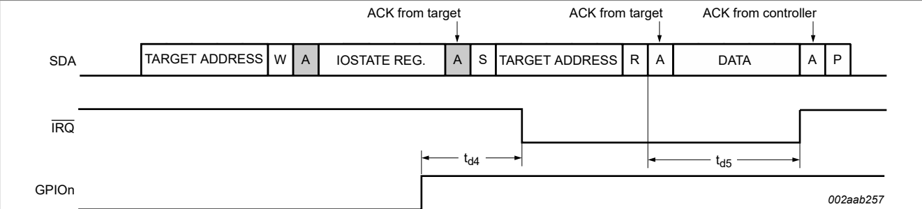
Figure 30. GPIO pin interrupt (SC16IS750 and SC16IS760 only)
