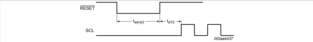
Figure 26. SCL delay after reset
