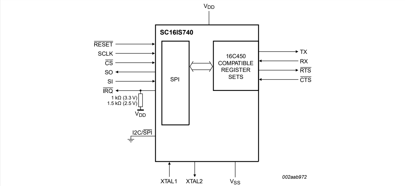
Figure 4. Block diagram of SC16IS740 SPI interface
