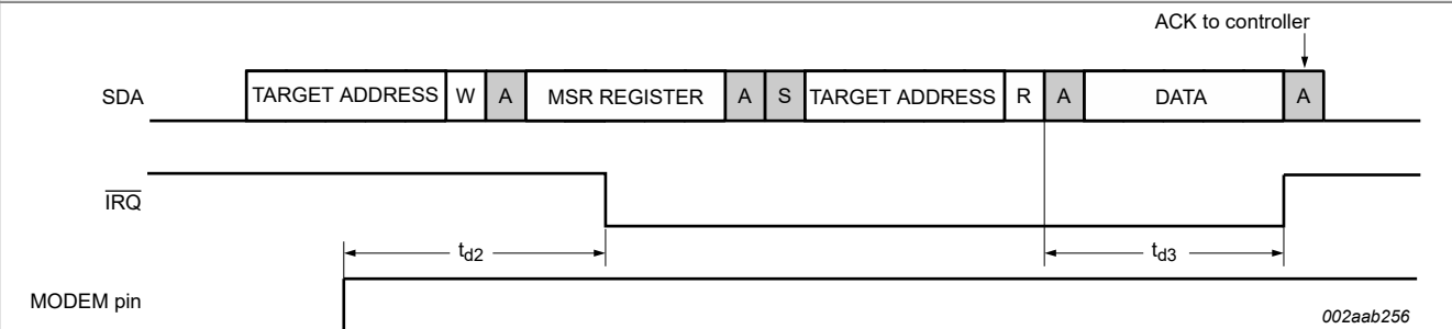
Figure 29. Modem input pin interrupt (SC16IS750 and SC16IS760 only)
