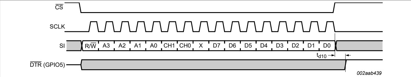
Figure 37. SPI write MCR to DTR output switch (SC16IS750 and SC16IS760 only)
