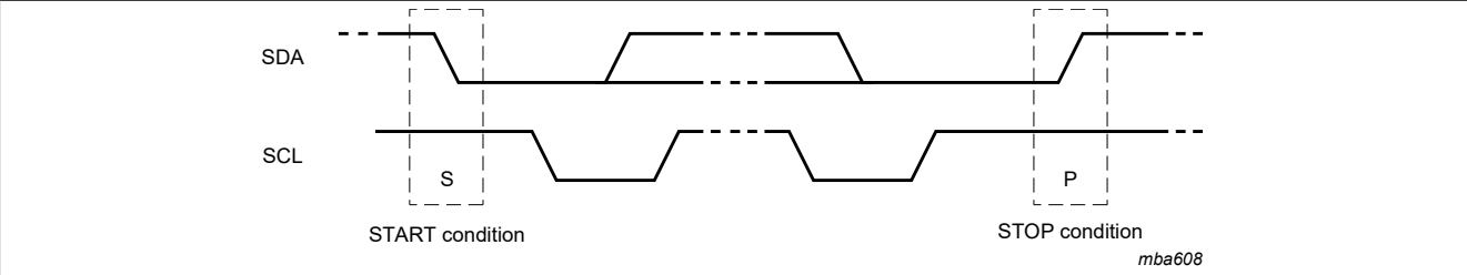
Figure 18. START and STOP conditions
