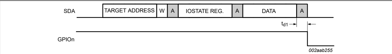
Figure 28. Write to output (SC16IS750 and SC16IS760 only)
