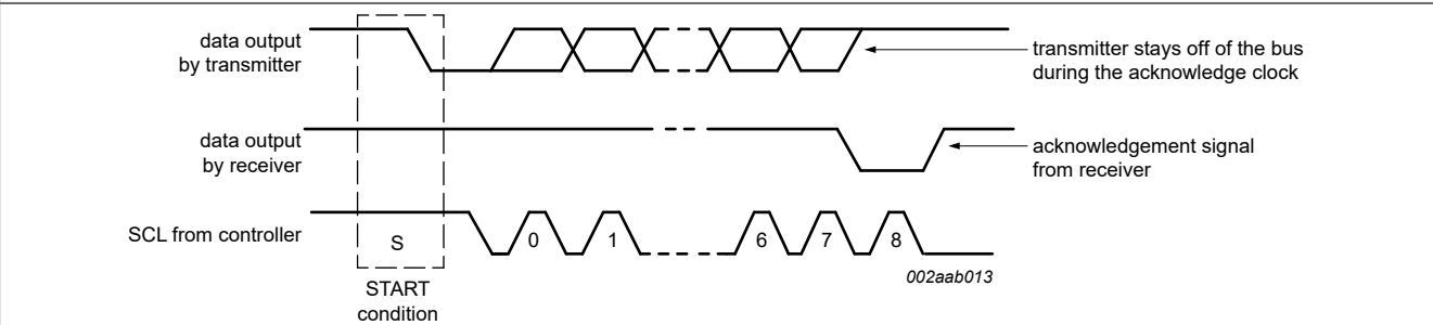
Figure 20. Acknowledge on the I 2 C-bus
