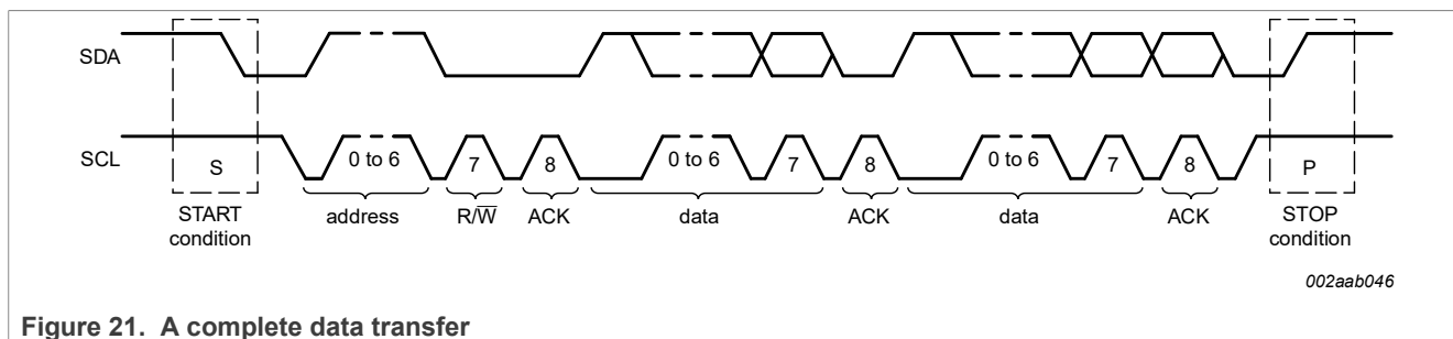
Figure 21. A complete data transfer
