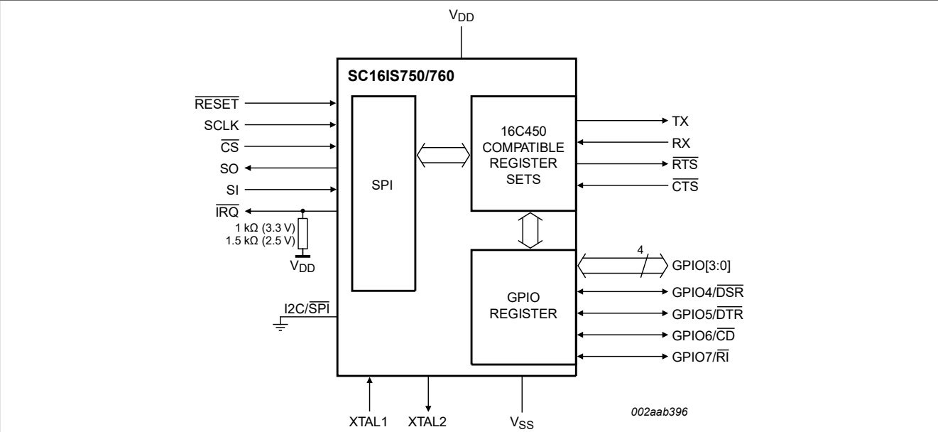
Figure 3. Block diagram of SC16IS750/760 SPI interface
