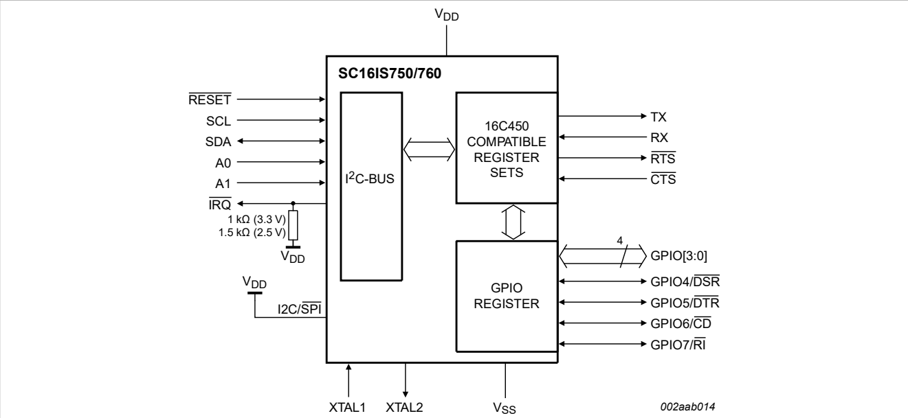
Figure 1. Block diagram of SC16IS750/760 I 2 C-bus interface
