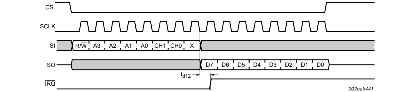
Figure 38. SPI write THR to clear TX INT
