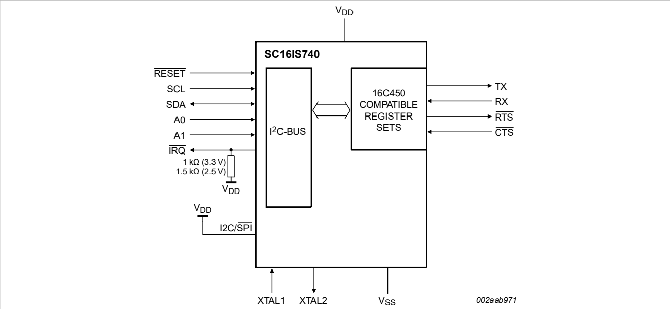
Figure 2. Block diagram of SC16IS740 I 2 C-bus interface
