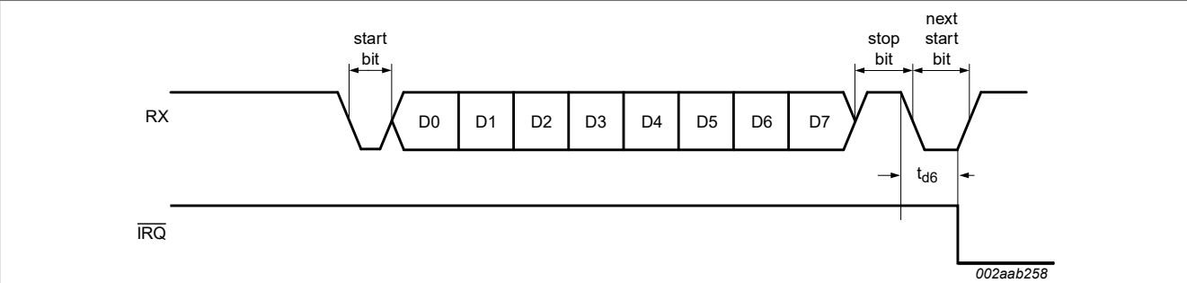
Figure 31. Receive interrupt
