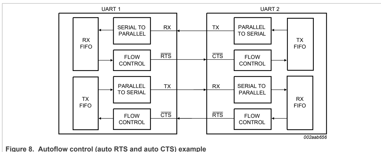
Figure 8. Autoflow control (auto RTS and auto CTS) example
