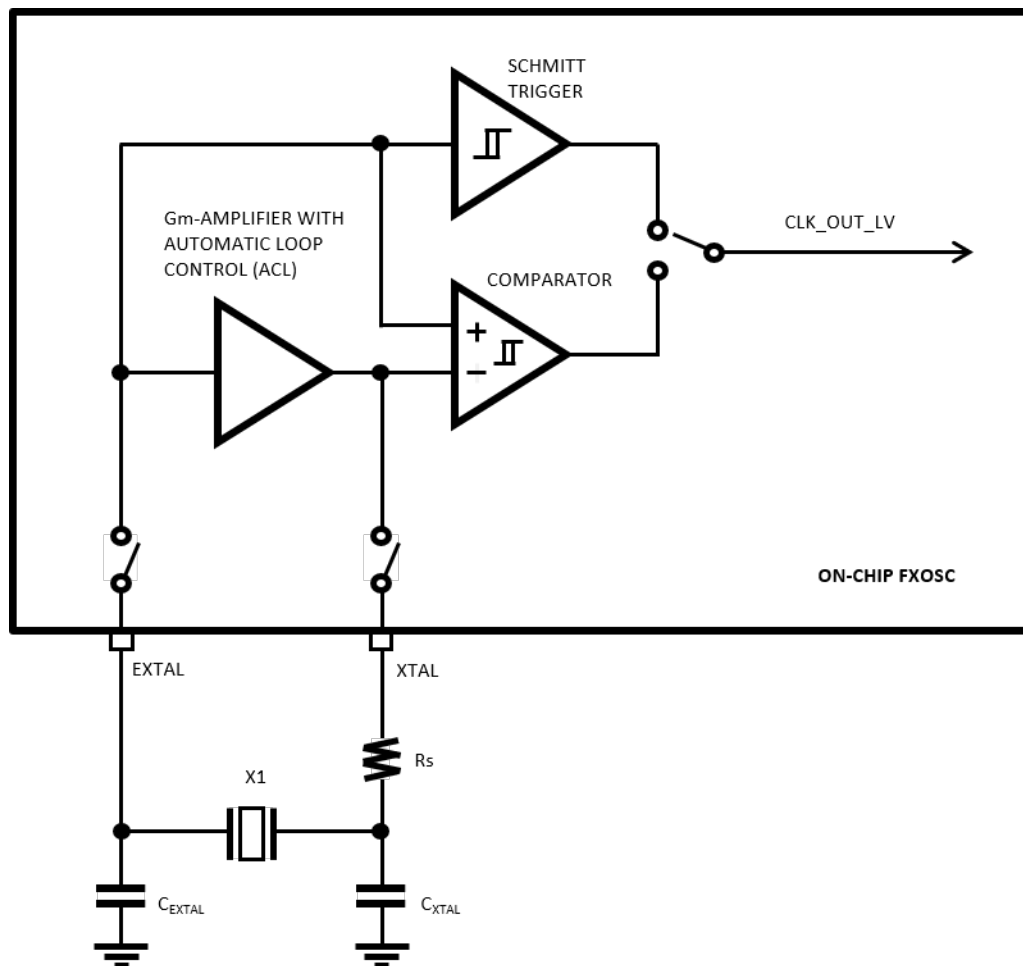
Figure 13. Block diagram
