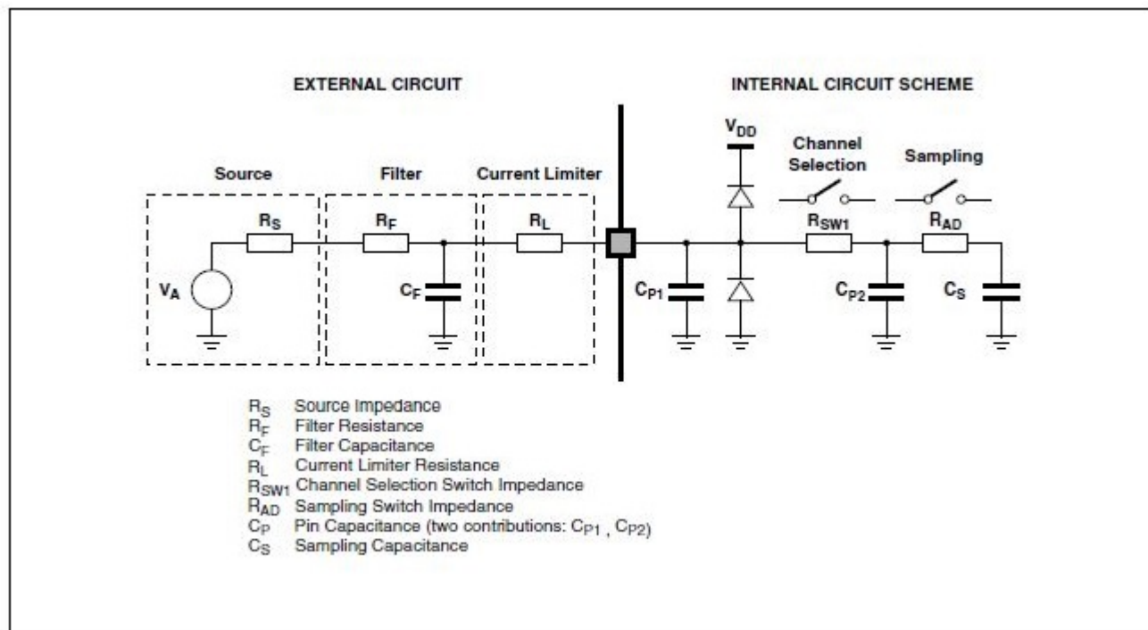
Figure 25. ADC input impedance equivalency diagram
