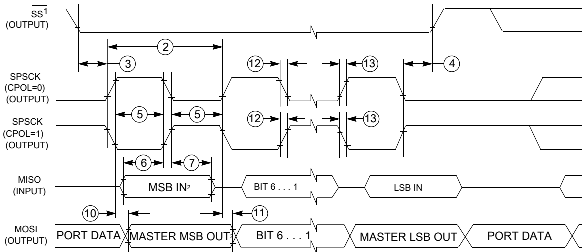
Figure 30. LPSPi master mode timing (CPHA = 0)
