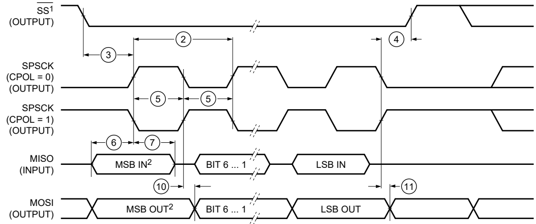
Figure 16. LPSPI Master Mode Timing (CPHA=0)
