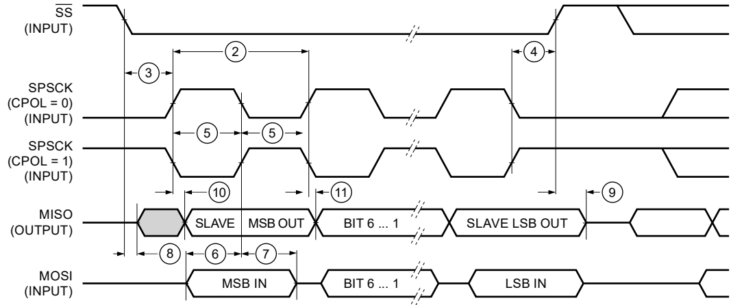
Figure 14. LPSPI Slave Mode Timing (CPHA=1)
