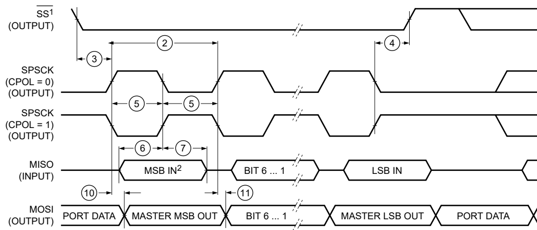
Figure 17. LPSPI Master Mode Timing (CPHA=1)
