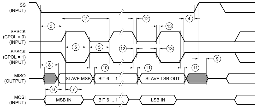
Figure 15. LPSPI Slave Mode Timing (CPHA=0)
