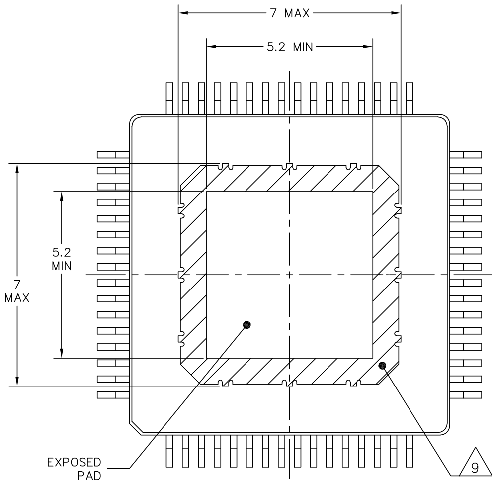
VIEW J-J
