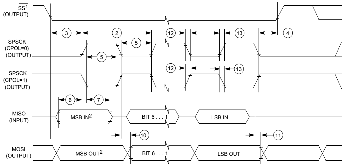
Figure 30. LPSPi master mode timing (CPHA = 0)
