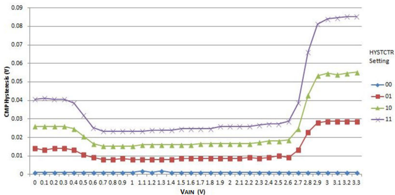
Figure 26. Typical hysteresis vs. V_{\text{AIN}} ( V_{\text{DDA}} = 3.3 \text{ V} , \text{PMode} = 0 )
