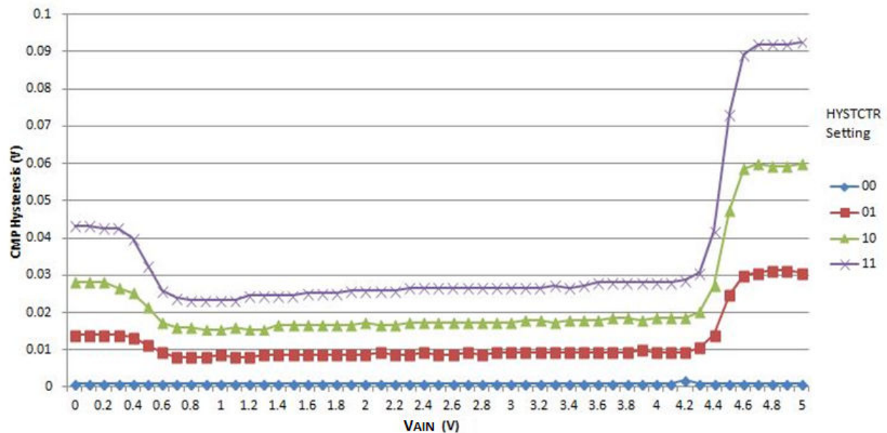
Figure 29. Typical hysteresis vs. V_{AIN} ( V_{DDA} = 5\text{ V} , PMODE = 1 )
