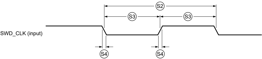
Figure 21. SWD Input Clock Timing
