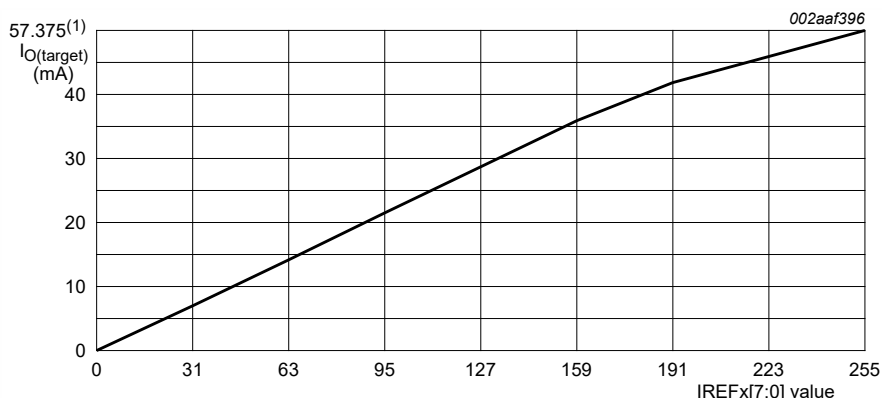
Figure 7. I O(target) versus IREFx value
