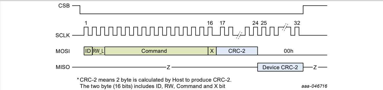
Figure 38. Two-byte command format with no return data
