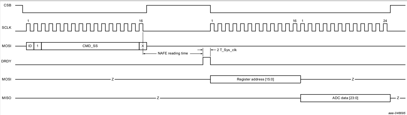
Figure 19. CMD_SS timing diagram with CSB high
