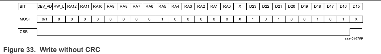
Figure 33. Write without CRC
