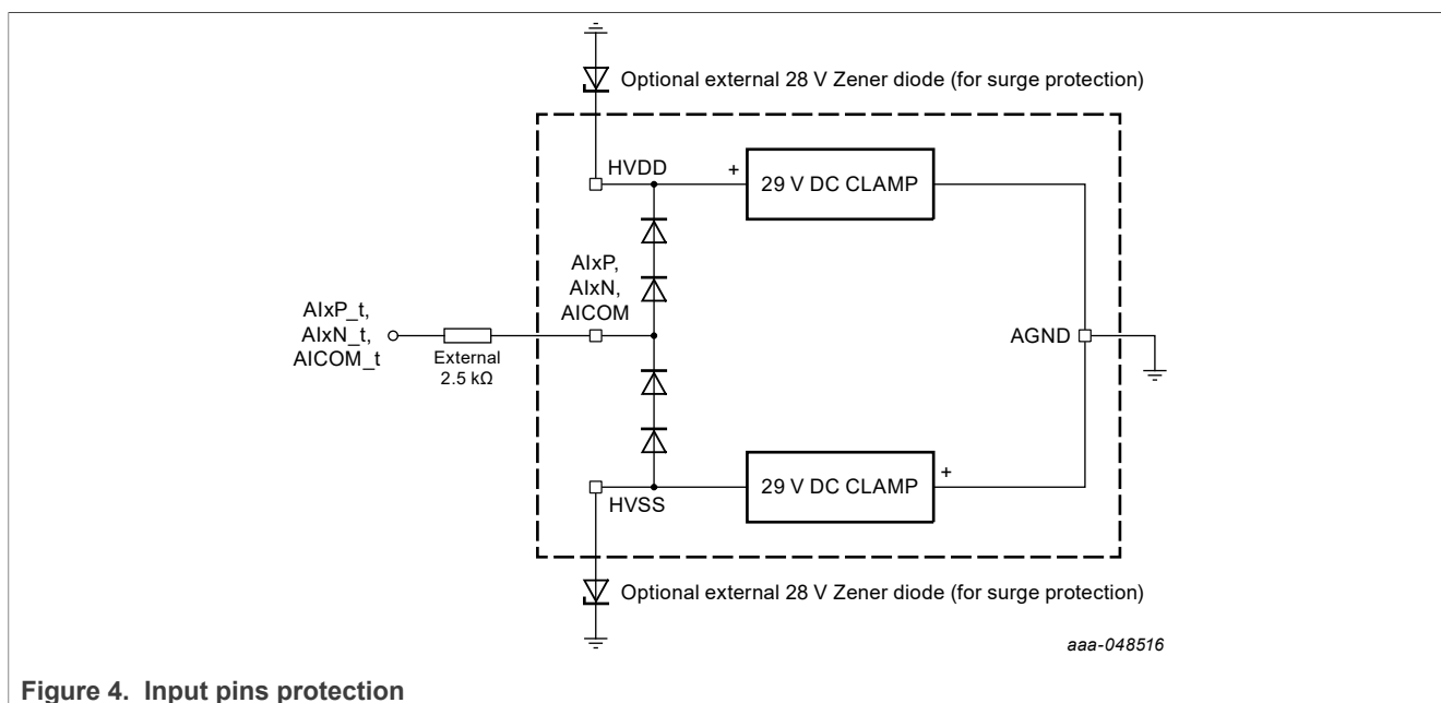
Figure 4. Input pins protection
