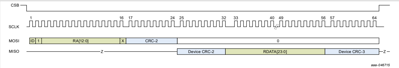
Figure 40. Regular read 24-bit data with CRC_EN = 1
