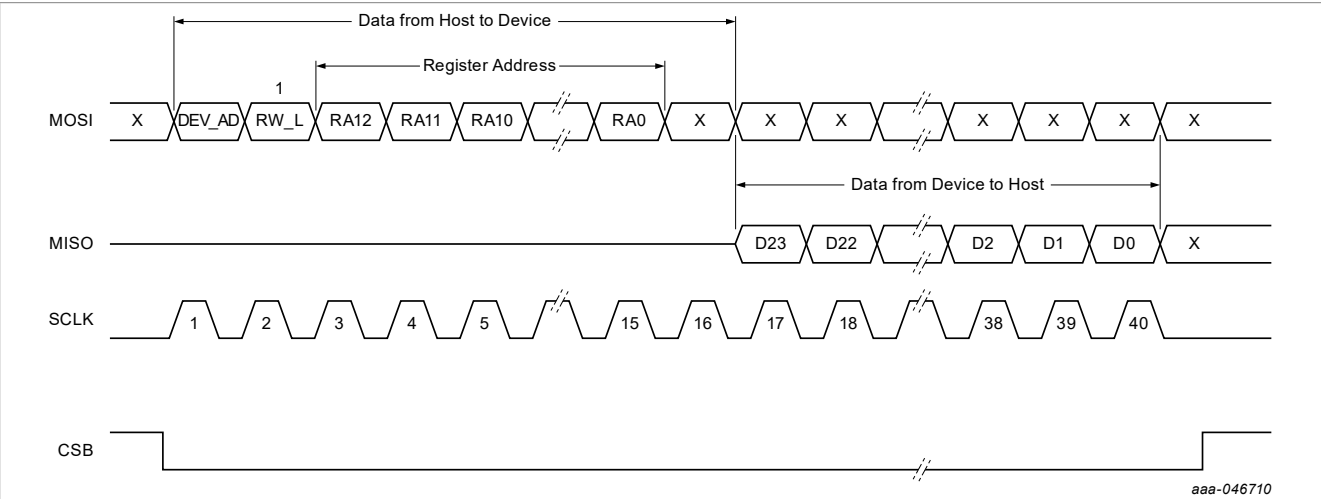
Figure 34. Read without CRC
