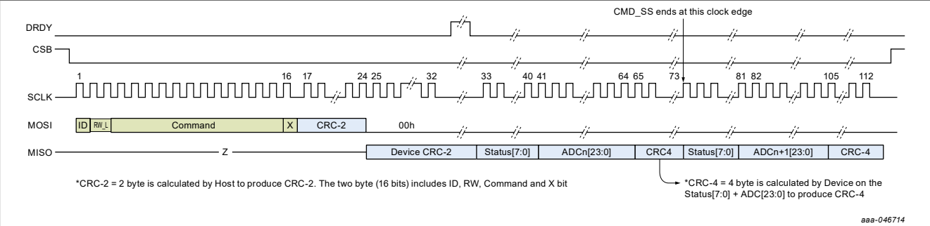
Figure 39. Conversion command data read operation 2/24-bit ADC, CRC_Enable = 1, Status_Enable = 0
