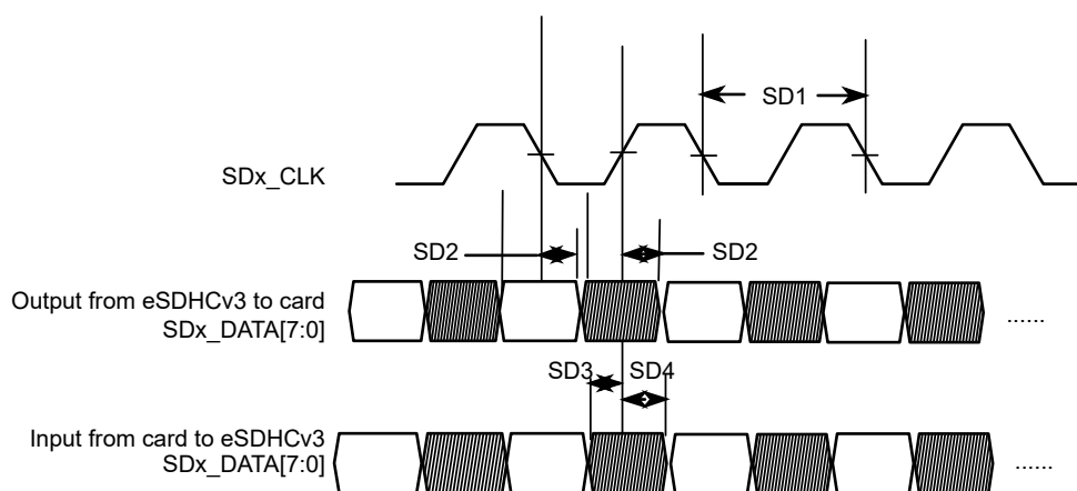
Figure 43. eMMC4.4/4.41 timing
