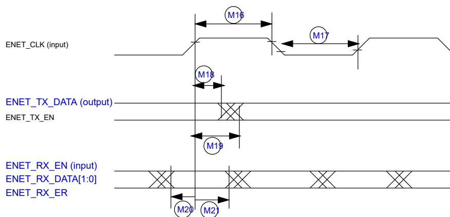
Figure 50. RMI mode signal timing diagram
