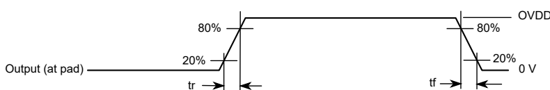
Figure 7. Output transition time waveform
