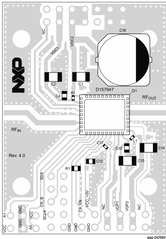
Figure 3. A3M39SL039 reference circuit component layout
