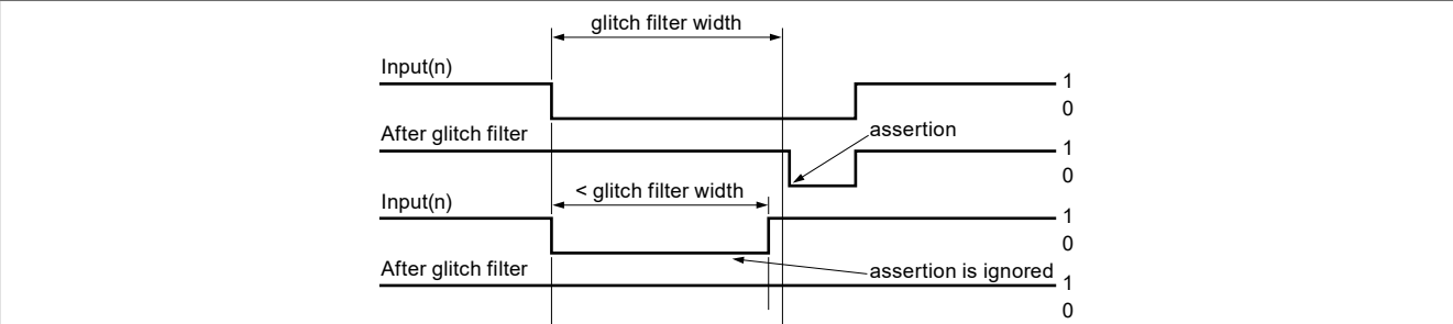
Figure 14. Digital filter
