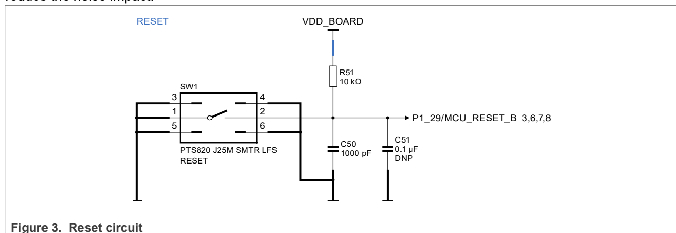
Figure 3. Reset circuit
