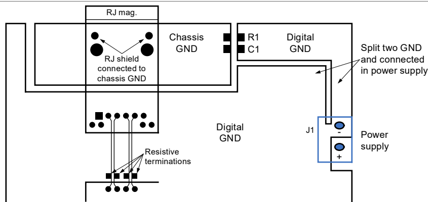
Figure 11. Shield connection example
