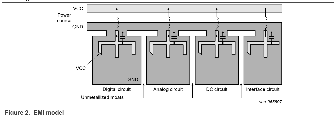
Figure 2. EMI model
