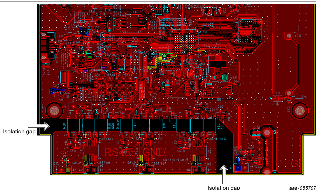
Figure 12. RS485 IO isolation circuit
