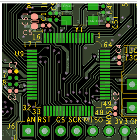
Figure 10. Decoupling capacitors and bypass circuit placement and return paths
