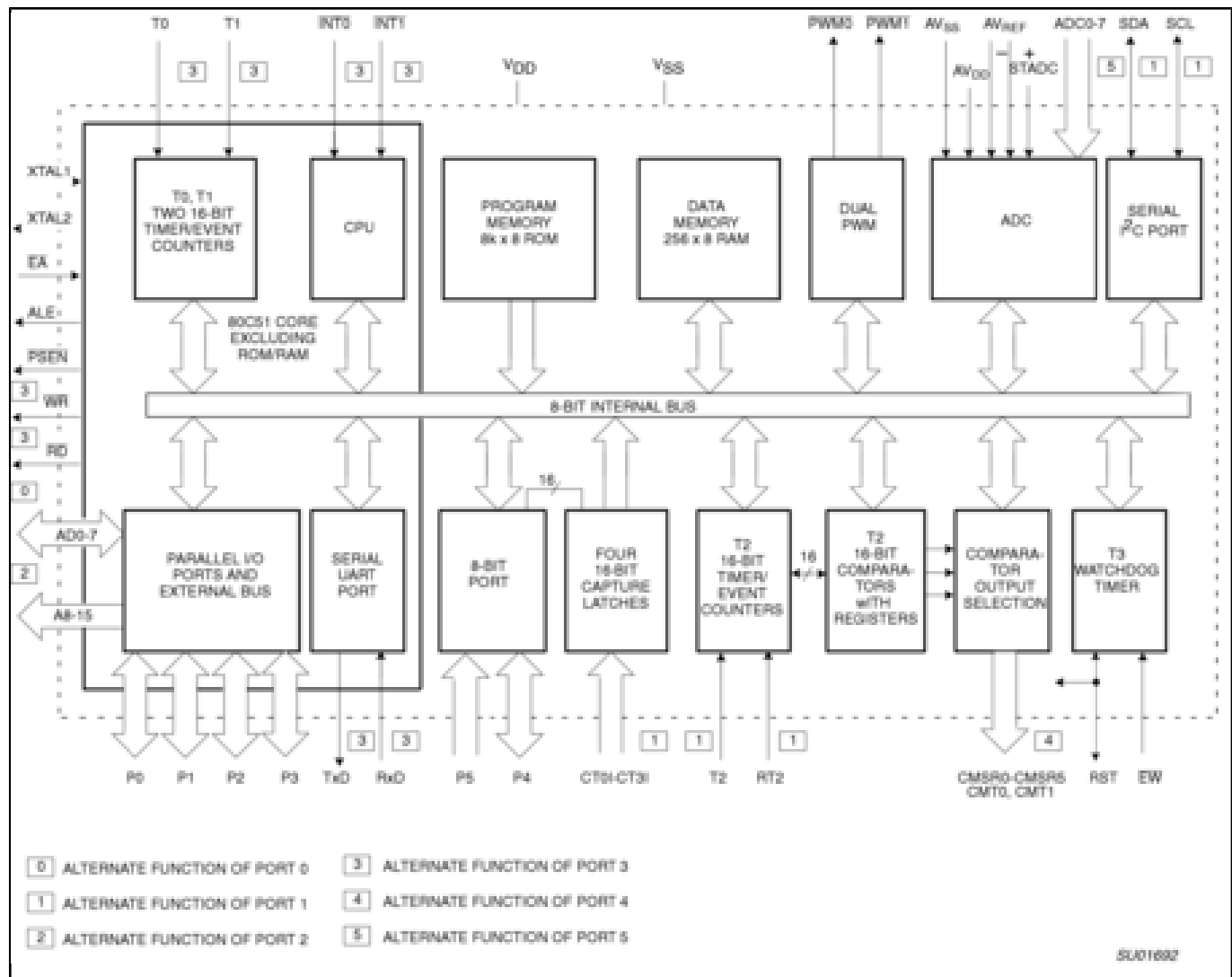
Block diagram: P80C552EBA, P80C552EBB, P80C552EFA, P80C552EFB, P80C552IBA, P80C552IFA, P83C552EFA Block Diagram
