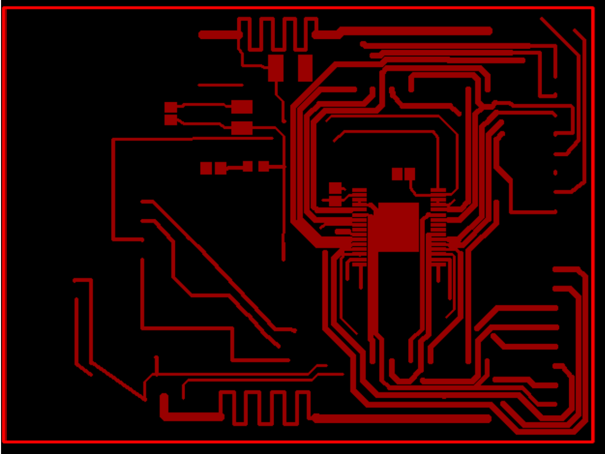
Figure 11. PCB Top
