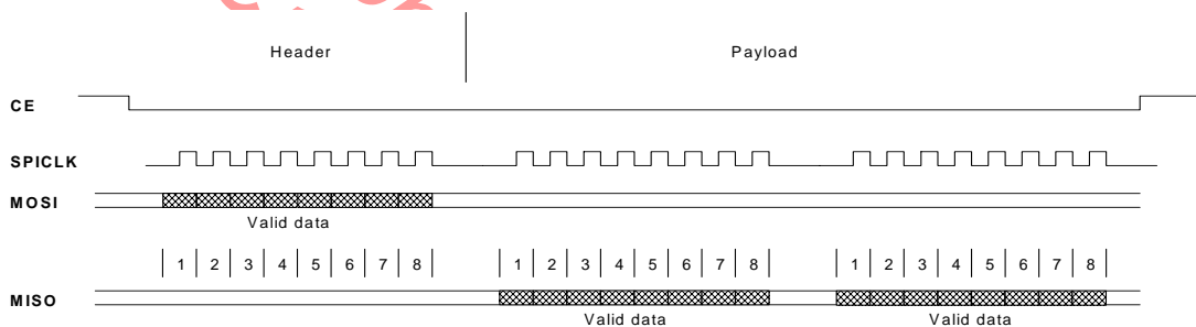
Figure 5-3. Singular Read Access
