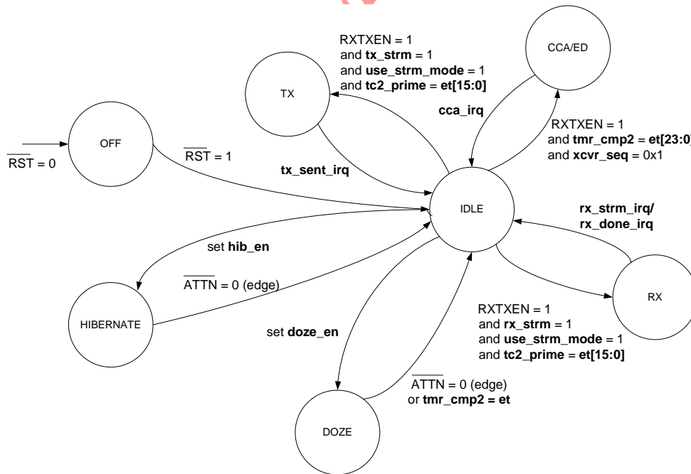
Figure 6-4. State Diagram for Stream Mode With TC2_Prime Enabled State ( \text{tmr\_trig\_en} = 1 )
