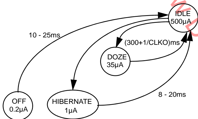
Figure 3-4. MC13192 Modem Low Power Recovery Times
