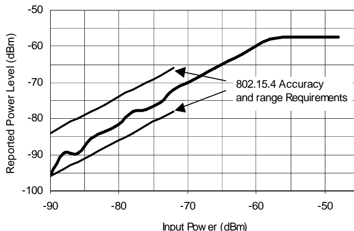
Figure 6-6. CCA Reported Power Level vs. Input Power
