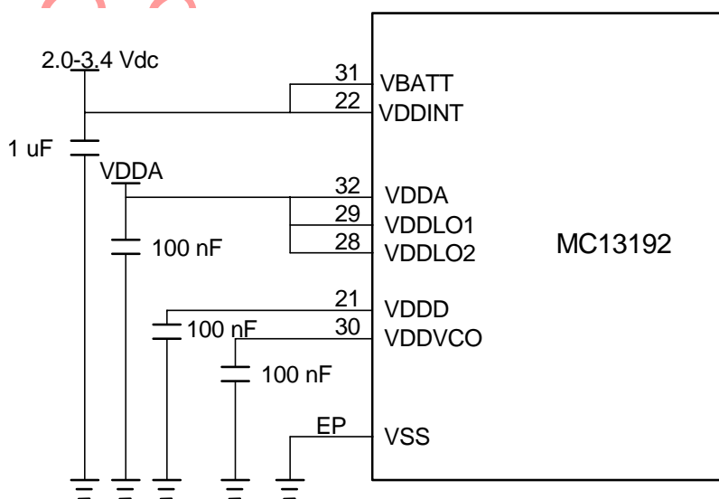
Figure 3-1. MC13192 Power Supply Connections
