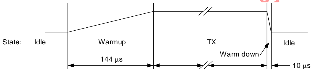
Figure 3-7. TX Timing Profile
