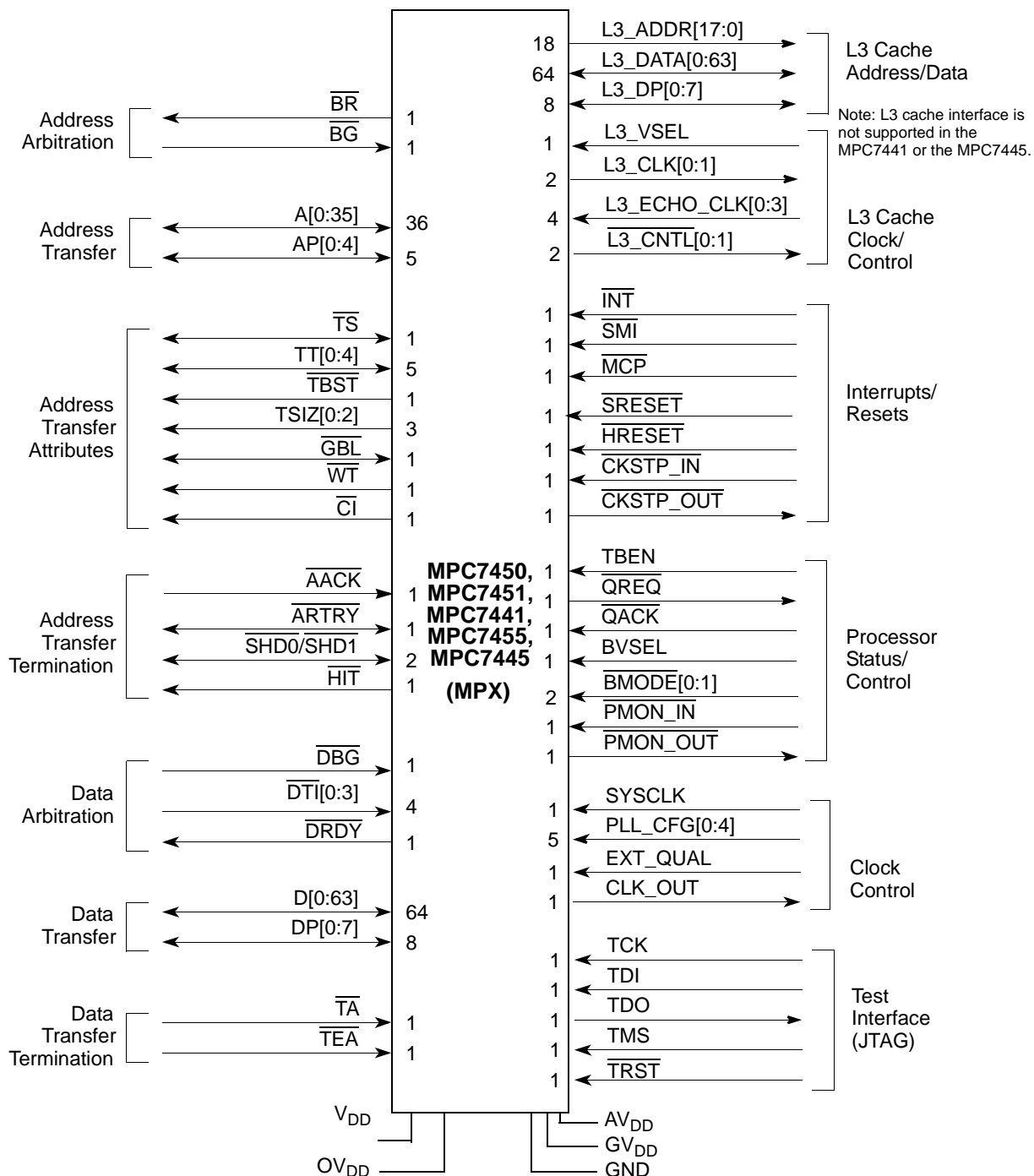
Figure 7. MPX Bus Signal Groups in the MPC7450, MPC7451, MPC7441, MPC7455, and MPC7445
