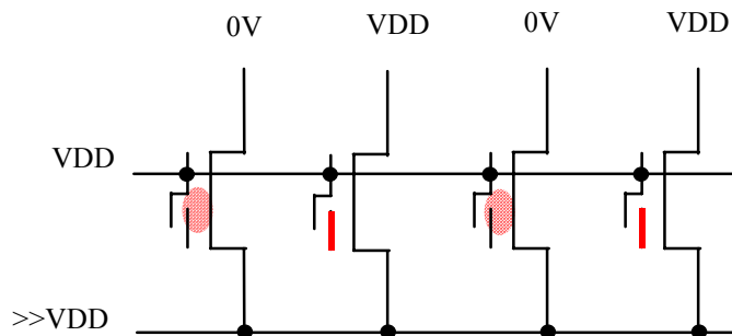
Figure 3. Programming a '0101' pattern into Split-Gate Flash
